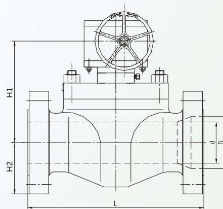
Gear Operator
