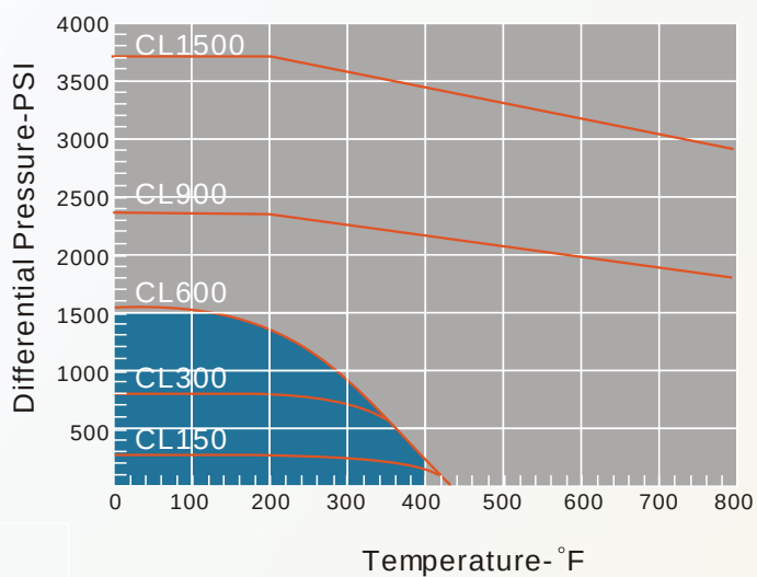
Teflon Seats
