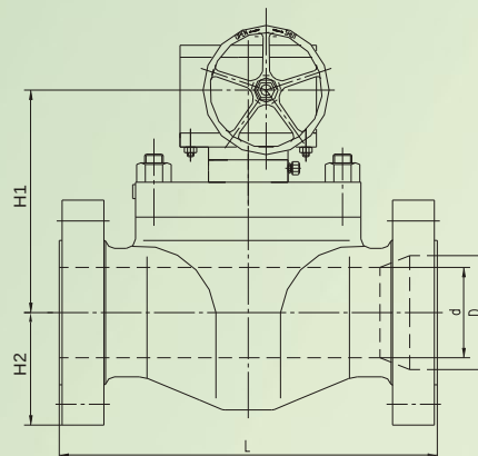
Gear Operator
