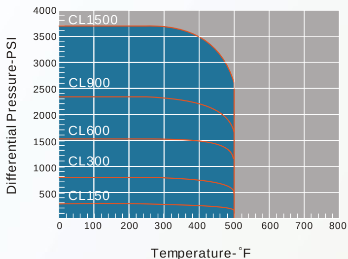
PEEK Seats
