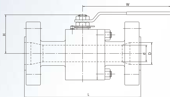
Reduced Port
