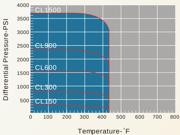
Glass-filled PTFE Seats
