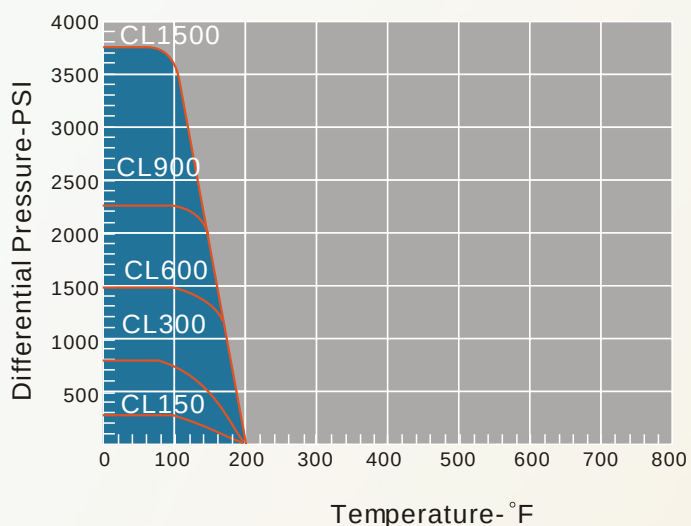
Delrin Seats
