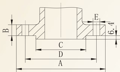
600LB and 900LB Steel
