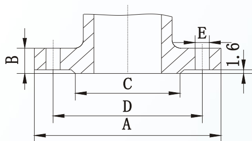
150 and 300 LB Steel
